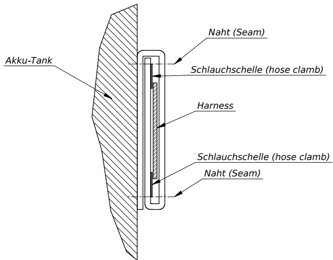
Figure 2.1: Belt Loop
